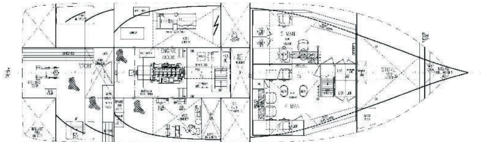
BELOW DECK
